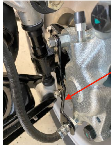
Brake caliper and hose locking plate
