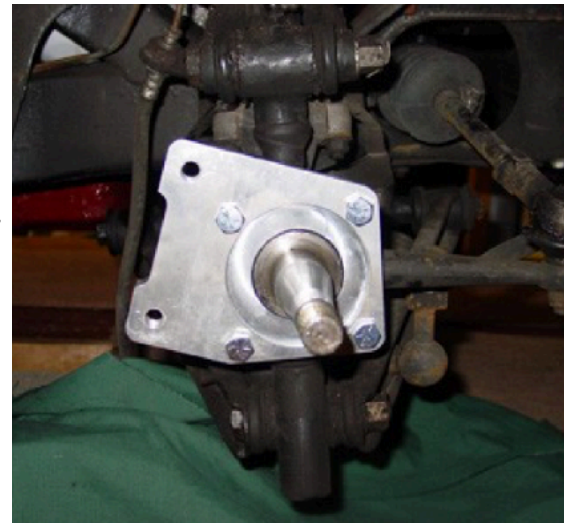
Caliper adaptor plate bolted on [Note: These are Left & Right Handed]
