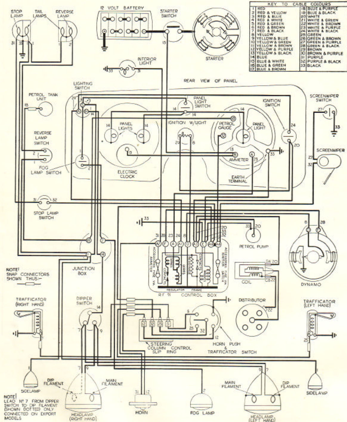
Illustration No. N.26. Diagram of the wiring system, with RF.91 Control Unit. (Chassis Numbers Y.0251 to Y.0583.)
